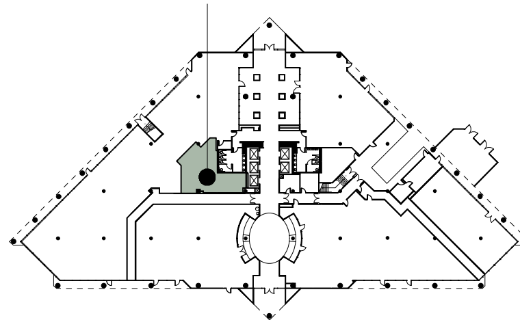
1ST FLOOR FLOOR KEY PLAN
